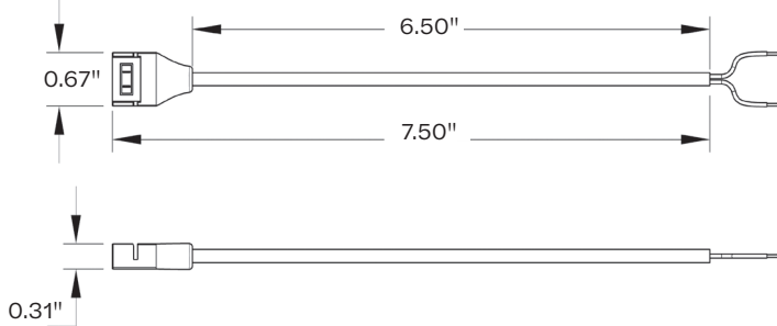
Single-color connector with 6" wire whip
