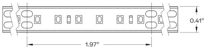
Single-color cut section
