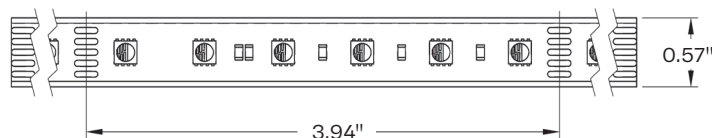
RGBW cut section
