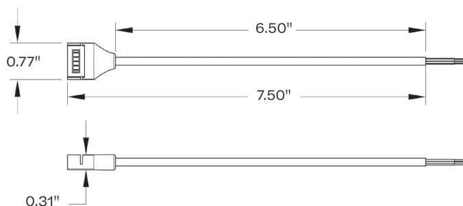
RGBW connector with 6" wire whip
