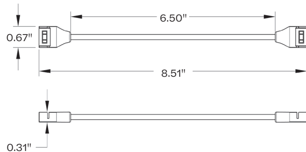
Single-color 6" jumper connector
