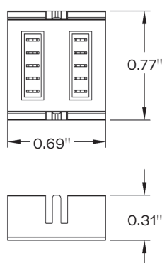
RGBW middle connector
