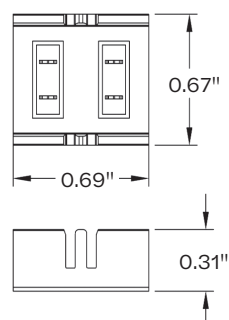
Single-color middle connector
