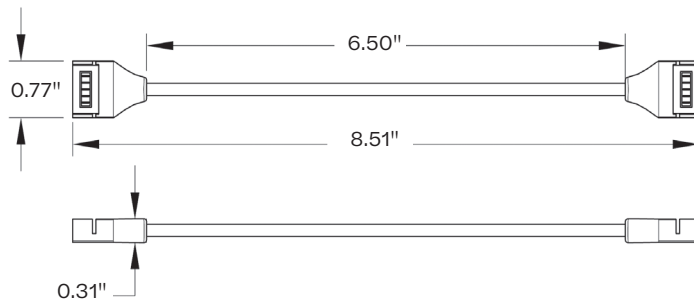
RGBW 6" jumper connector
