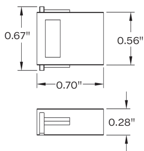
Single-color end cap
