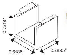
Transparent PC clips* A-SXMH-CLPL
