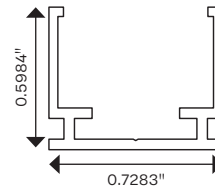
Aluminum mill finish clips for outdoor applications A-SXMH-CLAL
